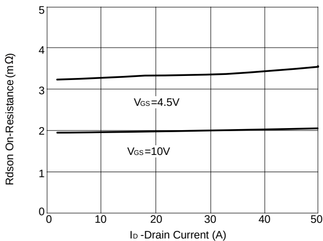
Figure 5: Rdson-Drain Current
