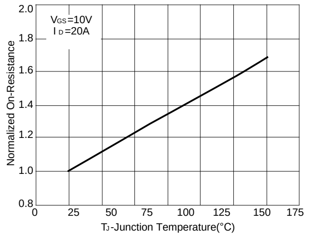
Figure 2: Rdson-Junction Temperature
