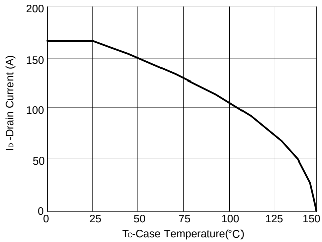
Figure 9: Current De-rating
