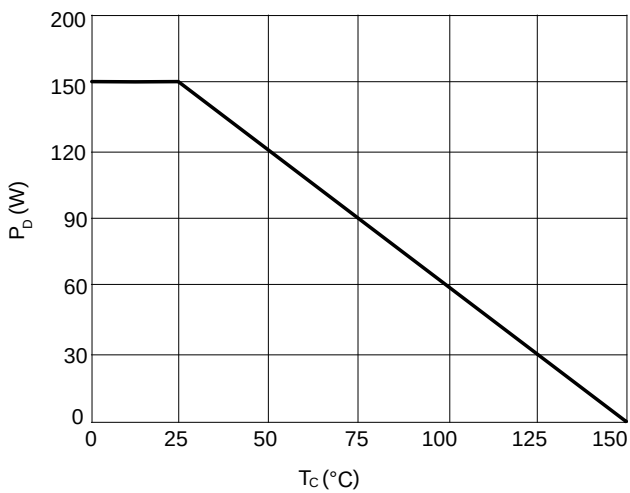
Figure 11: Power De-rating
