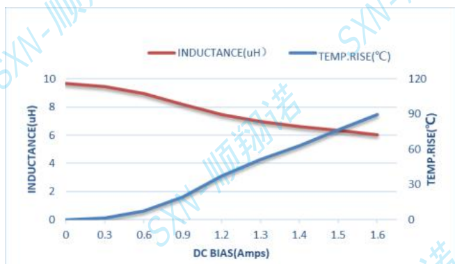
SMTC201210-100M
