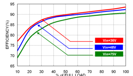
FED40-48S05 Efficiency VS Output Load
