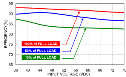
FED40-48S05 Efficiency VS Input Voltage
