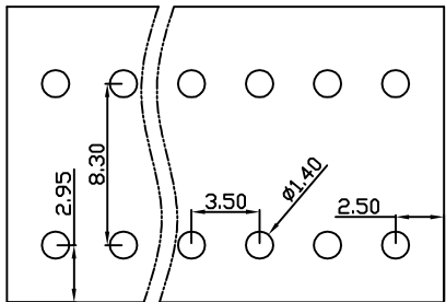
PCB Layout
