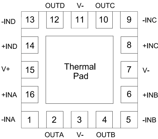
QFN2*2-16L
