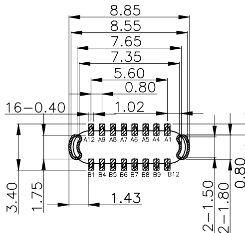
RECOMMENDED PCB LAYOUT COMPONENT SIDE(GENERAL TOLERANCE:±0.05)
