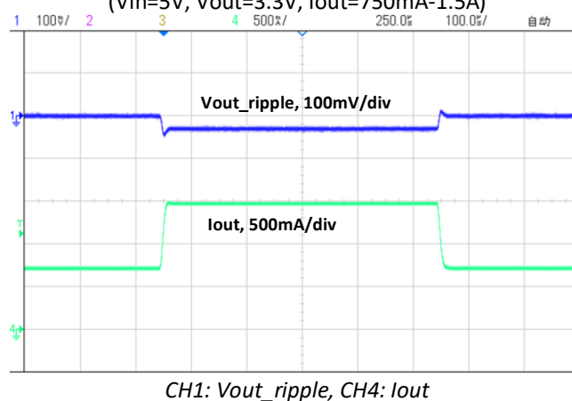
Load Transient Response ( V_{in}=5V , V_{out}=3.3V , I_{out}=750mA-1.5A )
