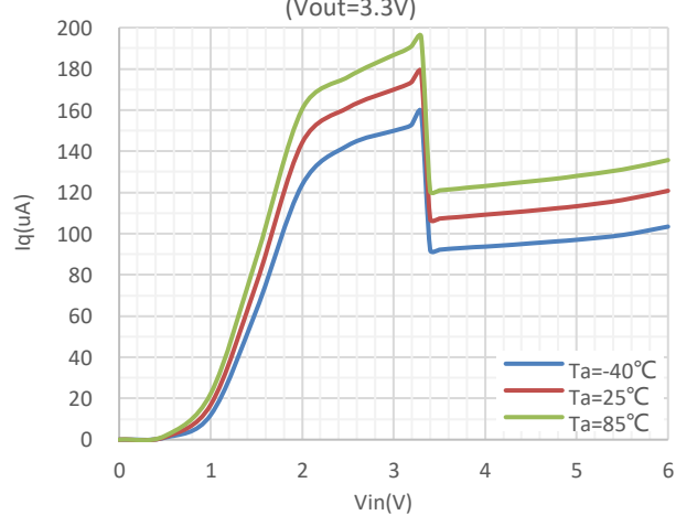
Iq (Vout=3.3V)
