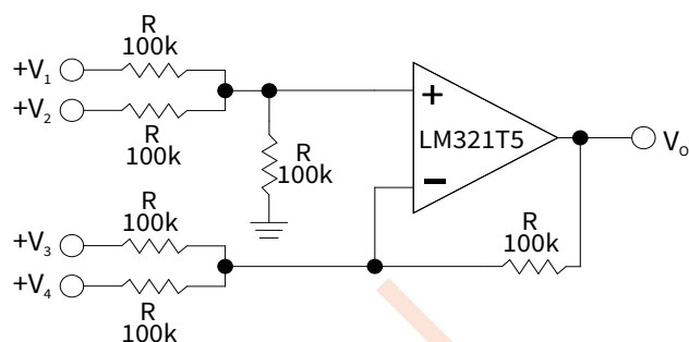
DC Summing Amplifier ( V_{IN'S} \geq 0 V_{DC} and V_o \geq V_{DC} )
