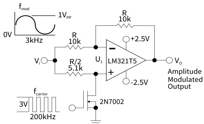
Amplitude Modulator Circuit
