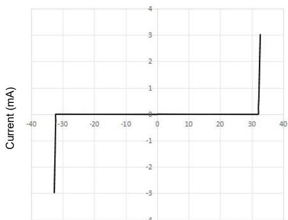
V_R Voltage vs Current
