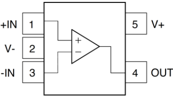
SOT23-5_B/SOT353_B
