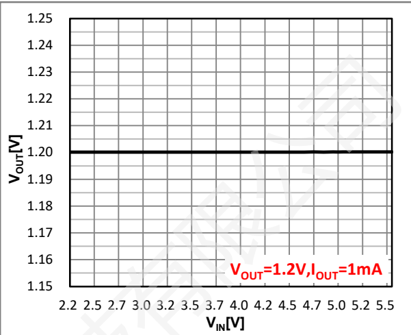
Figure 14. Line Regulation
