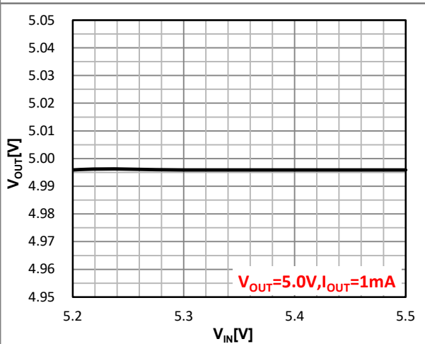
Figure 18. Line Regulation
