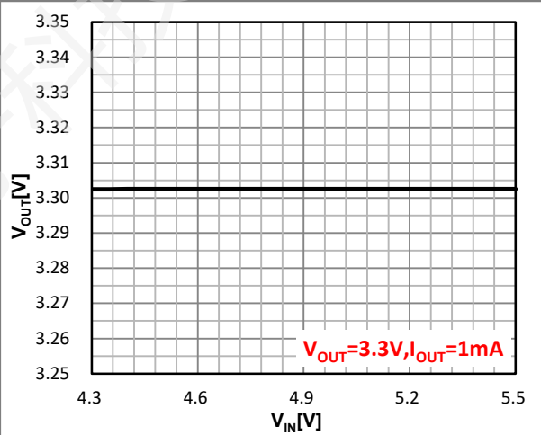
Figure 16. Line Regulation
