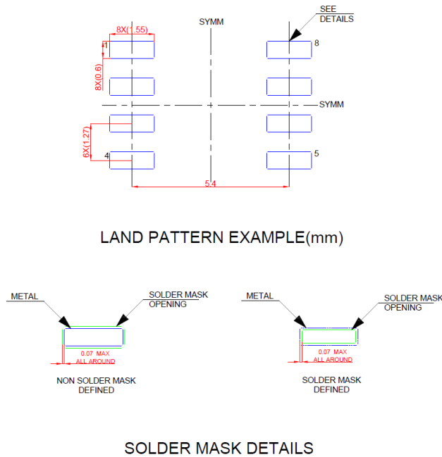
Figure 9.2 SOP8 Package Board Layout Example
