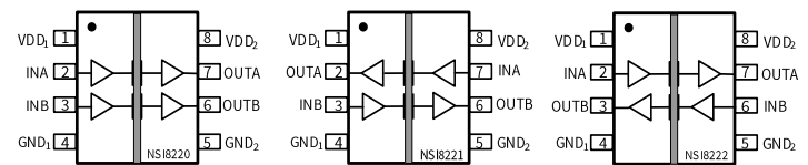
Figure 1. NSI822xC SOP8 Block Diagram
