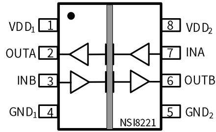
Figure 1.5 NSI8221Cx SOW8 Package
