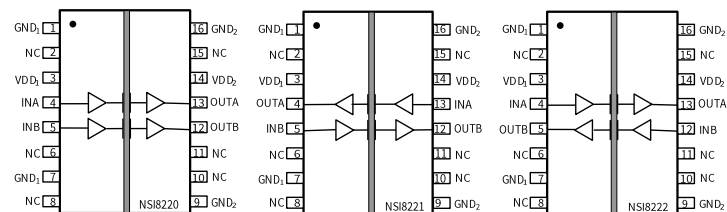
Figure 3. NSI822xC SOW16 Block Diagram
