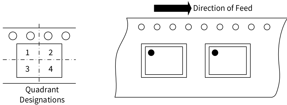
Figure 12.3 Tape Information of SOW8
