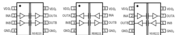
Figure 2. NSI822xC SOW8 Block Diagram
