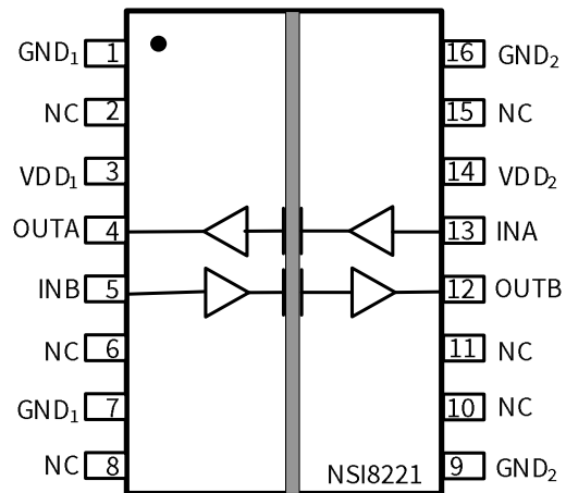
Figure 1.8 NSI8221Cx SOW16 Package
