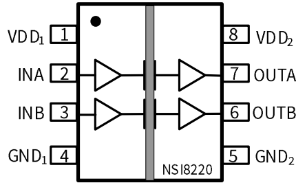
Figure 1.1 NSI8220Cx SOP8 Package
