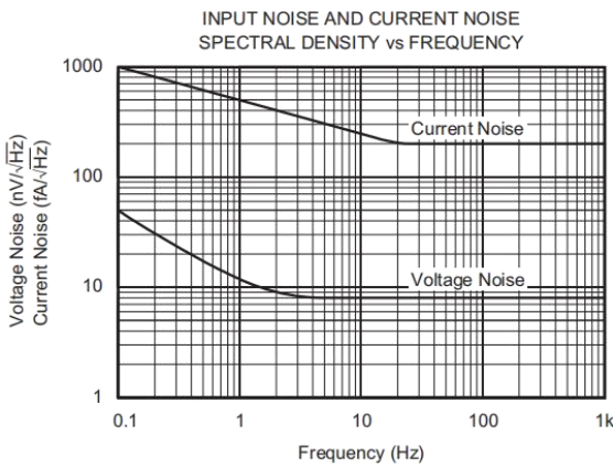
Figure 3. Input Noise and Current Noise Spectral Density vs Frequency
