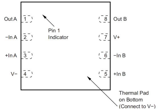
8-Pin DFN
