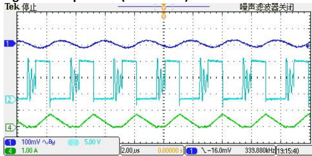
Light Load Operation(0.3A LOAD)
