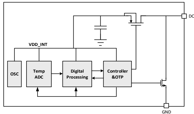
Figure 4.1 NST1001HA Functional Block Diagram
