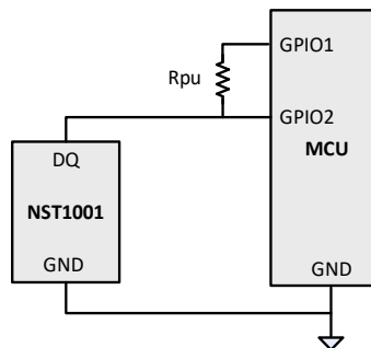
Figure 5.2 No power consumption in standby mode application
