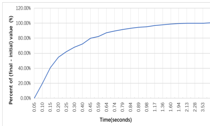
Figure 3.2 Thermal Response in stilling Oil (DFN-2L)
