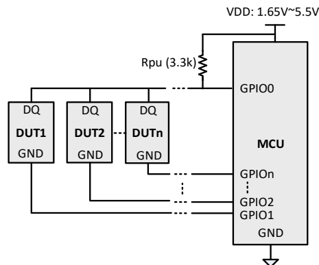
Figure 5.4 Multi-point temperature acquisition with NST1001HA
