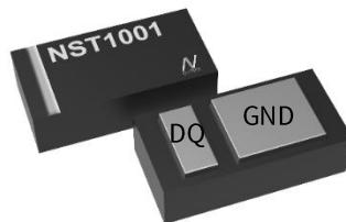
Figure 6.1 NST1001HAHA DFN-2L package
