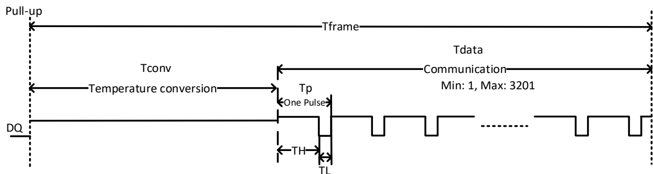
Figure 2.1 Timing Diagram
