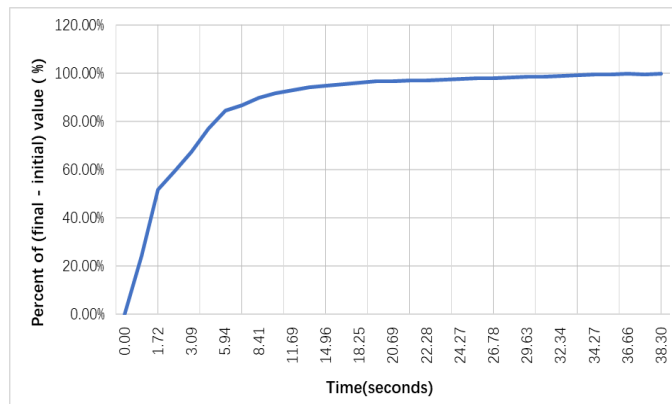
Figure 3.1 Thermal Response in stilling Air (DFN-2L)
