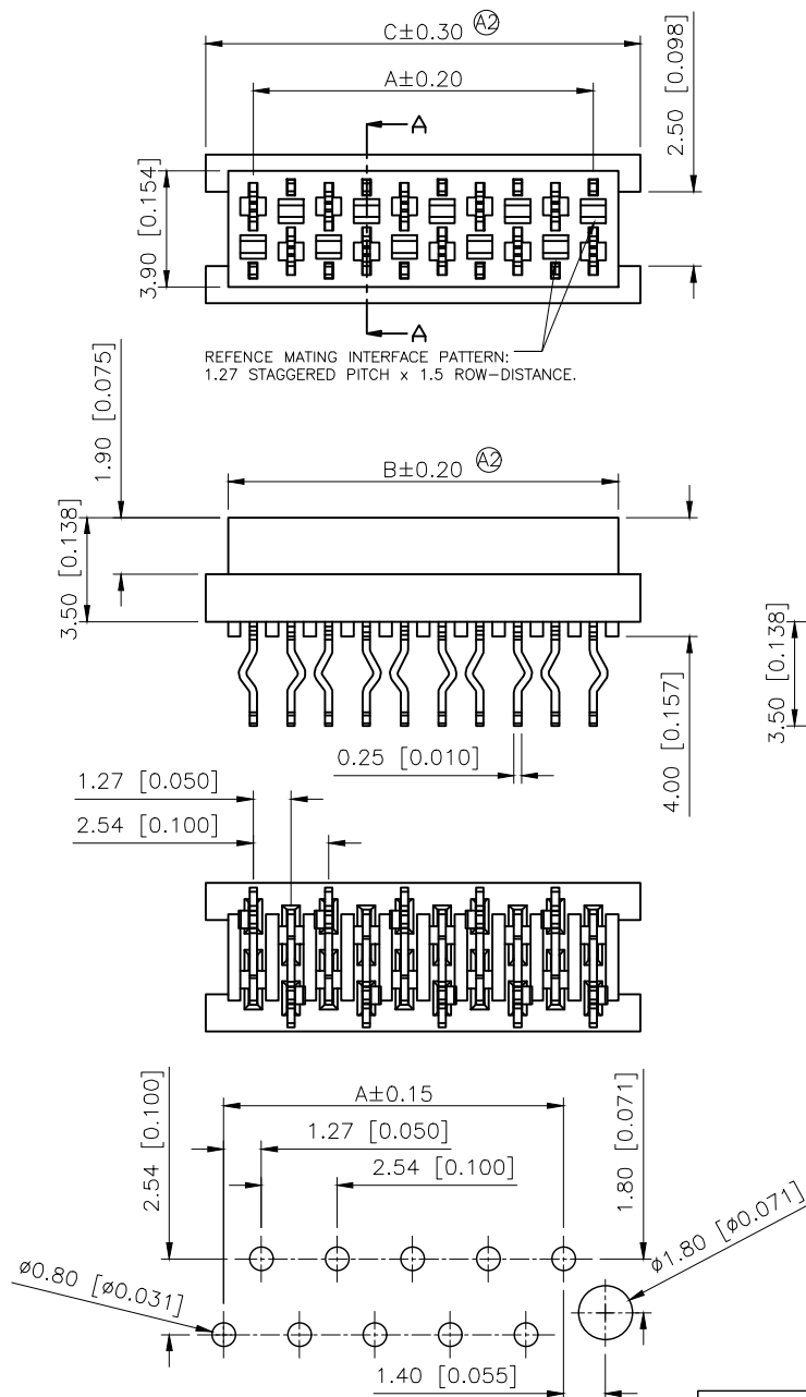
PCB Layout
