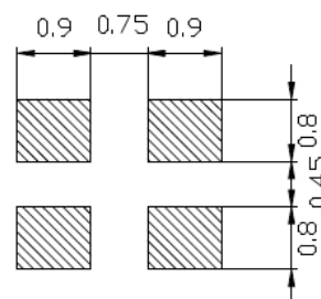
LAND PATTERN&lt;REFERENCE&gt;
