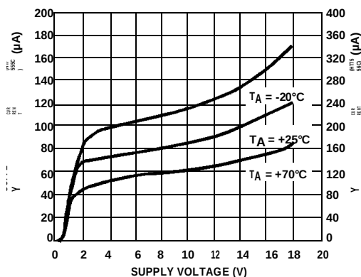
FIGURE 8. SUPPLY CURRENT vs SUPPLY VOLTAGE
