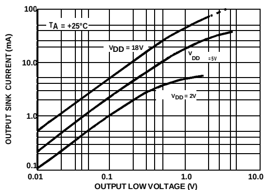
FIGURE 11. OUTPUT SINK CURRENT vs OUTPUT VOLTAGE
