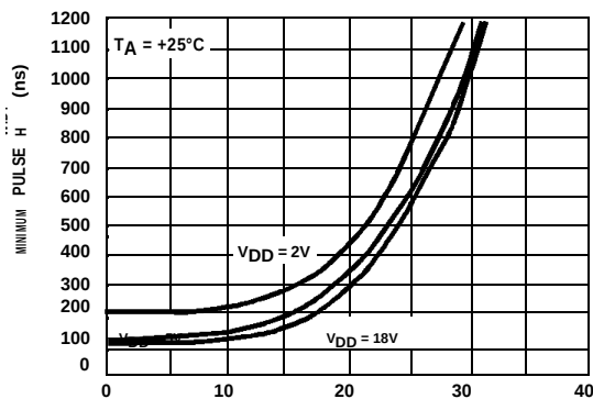
FIGURE 7. MINIMUM PULSE WIDTH REQUIRED FOR TRIGGERING
