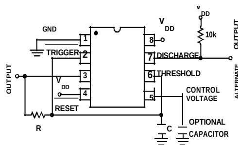
FIGURE 4. ASTABLE OPERATION
