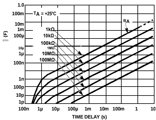
FIGURE 18. TIME DELAY IN THE MONOSTABLE MODE vs R_A AND C
