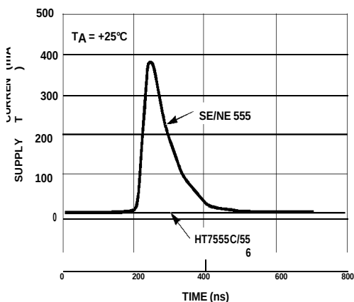
FIGURE 3. SUPPLY CURRENT TRANSIENT COMPARED WITH A STANDARD BIPOLAR 555 DURING AN OUTPUT TRANSITION
