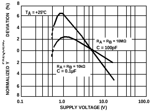
FIGURE 13. NORMALIZED FREQUENCY STABILITY IN THE ASTABLE MODE vs SUPPLY VOLTAGE
