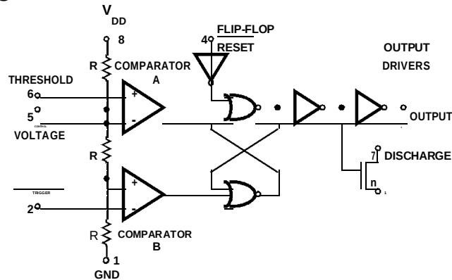
FIGURE 1. FUNCTIONAL DIAGRAM
