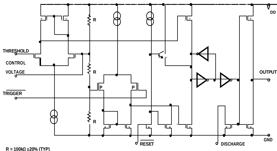
FIGURE 2. SCHEMATIC DIAGRAM
