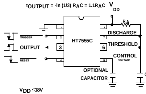
FIGURE 6. MONOSTABLE OPERATION
