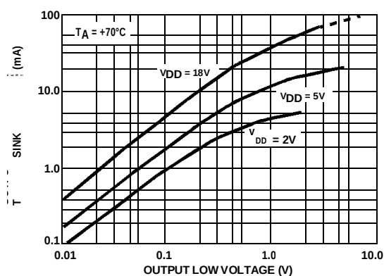
FIGURE 12. OUTPUT SINK CURRENT vs OUTPUT VOLTAGE
