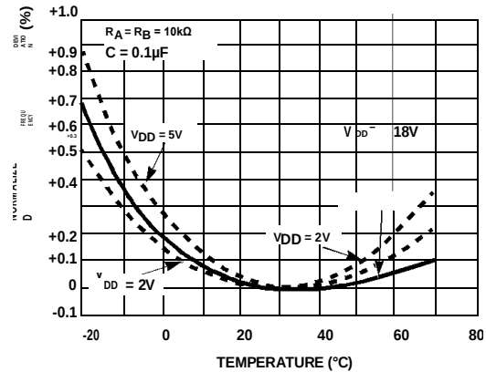
FIGURE 16. NORMALIZED FREQUENCY STABILITY IN THE ASTABLE MODE vs TEMPERATURE
