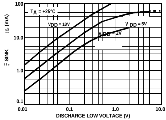
FIGURE 14. DISCHARGE OUTPUT CURRENT vs DISCHARGE OUTPUT VOLTAGE
