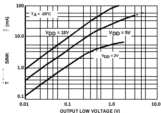
FIGURE 10. OUTPUT SINK CURRENT vs OUTPUT VOLTAGE
