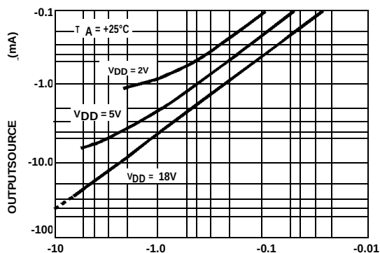
FIGURE 9. OUTPUT SOURCE CURRENT vs OUTPUT VOLTAGE
