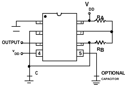
FIGURE 5. ALTERNATE ASTABLE CONFIGURATION
