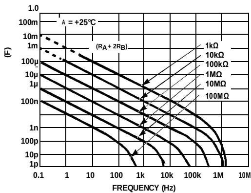
FIGURE 17. FREE RUNNING FREQUENCY vs R_A , R_B AND C
