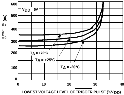
FIGURE 15. PROPAGATION DELAY vs VOLTAGE LEVEL OF TRIGGER PULSE
