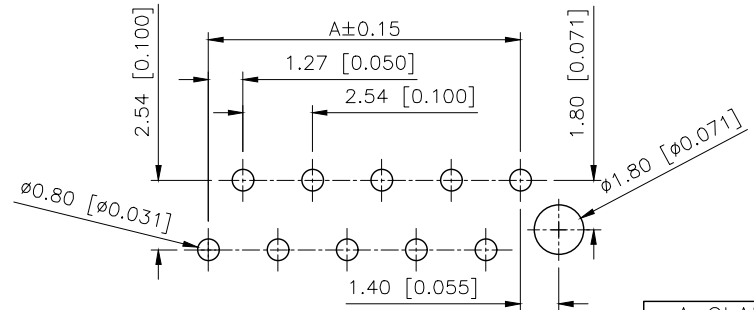
PCB Layout
