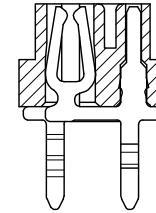
SECTION:A-A SCALE:1:1
