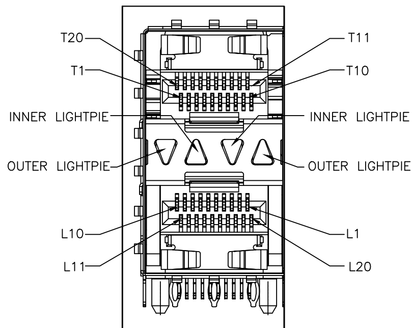
DETAIL A CIRCUIT NUMBERING AND LIGHTPIPE IDENTIFICATION
