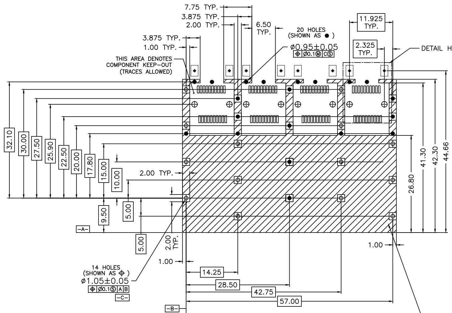
DETAIL H RECOMMENDED CONNECTOR LAYOUT 4X INDIVIDUALLY
