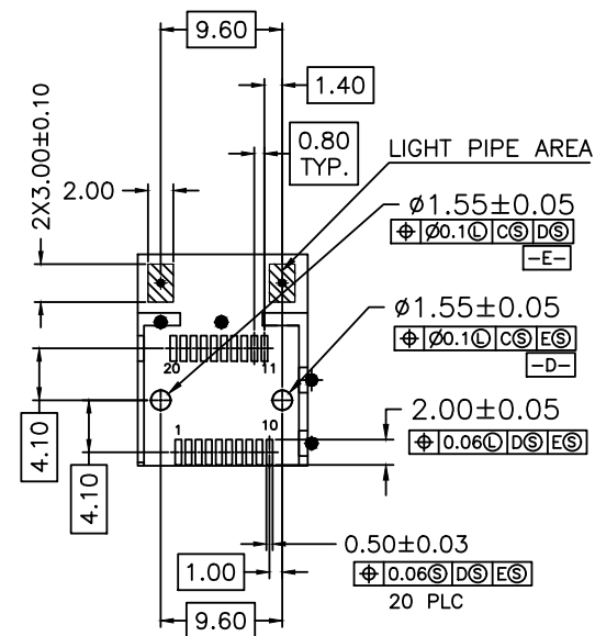
DETAIL H RECOMMENDED CONNECTOR LAYOUT 4X INDIVIDUALLY
