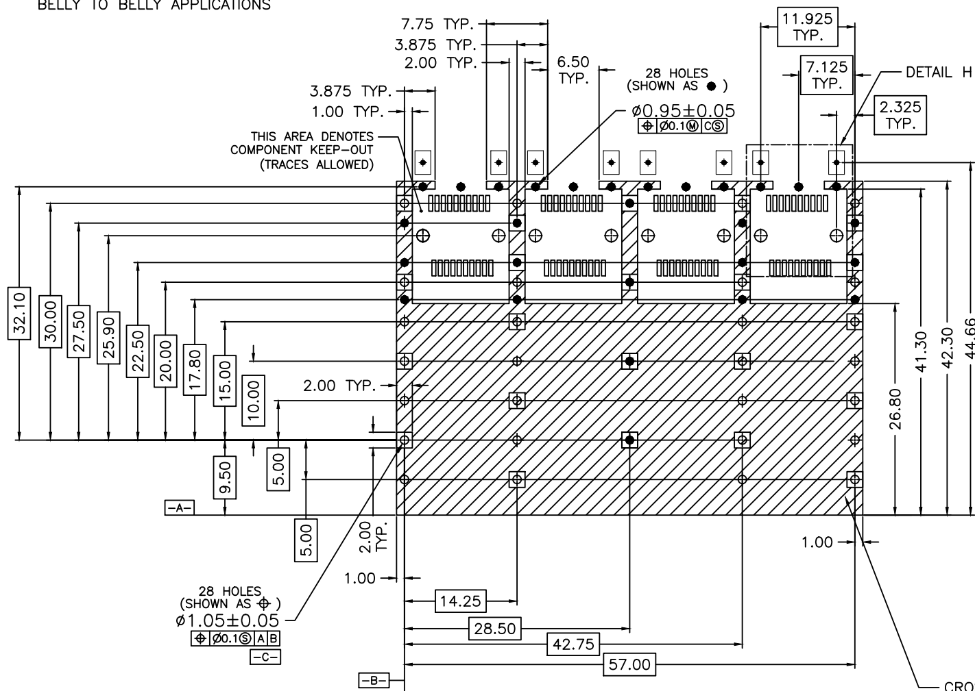
DETAIL H RECOMMENDED CONNECTOR LAYOUT 8X INDIVIDUALLY
