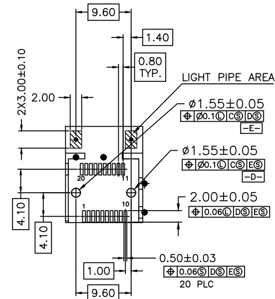
DETAIL H RECOMMENDED CONNECTOR LAYOUT 8X INDIVIDUALLY
