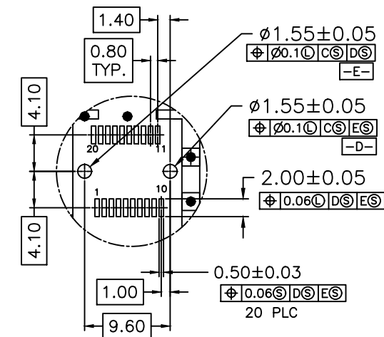
DETAIL H RECOMMENDED CONNECTOR LAYOUT 8X INDIVIDUALLY
