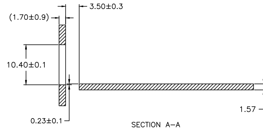
RECOMMENDED BEZEL DESIGN SINGLE SIDED APPLICATIONS
