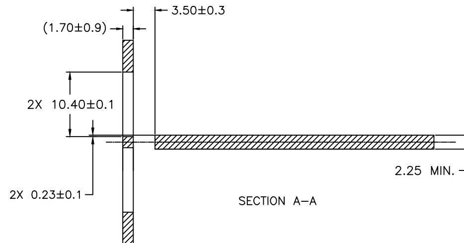
RECOMMENDED BEZEL DESIGN SINGLE SIDED APPLICATIONS
