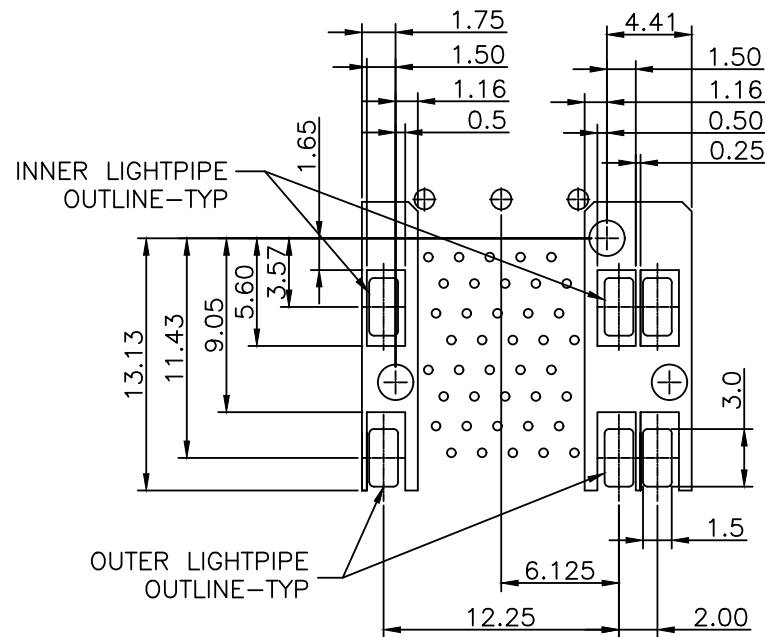
DETAIL-KEEPOUT ZONES
