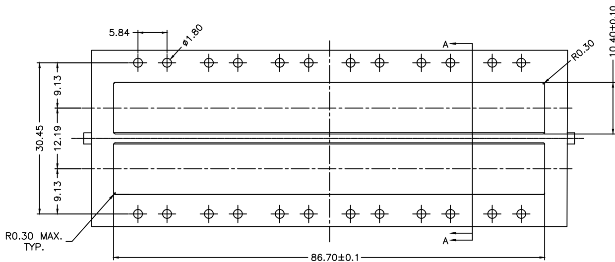
RECOMMENDED BEZEL DESIGN BELLY TO BELLY APPLICATIONS
