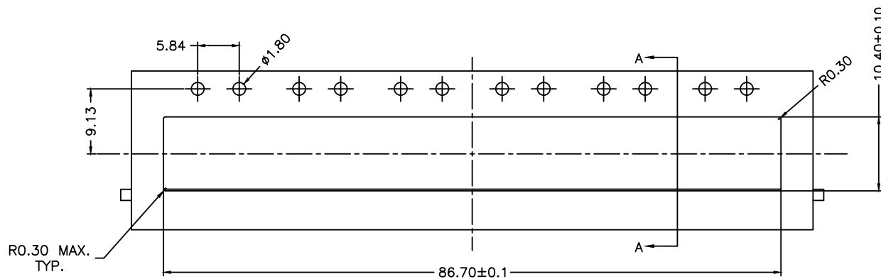
RECOMMENDED BEZEL DESIGN SINGLE SIDED APPLICATIONS
