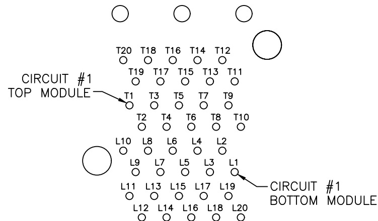
CIRCUIT NUMBERING COMPONENT SIDE OF BOARD
