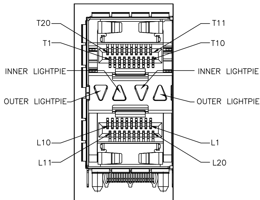
DETAIL A CIRCUIT NUMBERING AND LIGHTPIPE INDENTIRCATION
