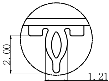
DETAIL A SCALE 5:1 QUANTITY:9
