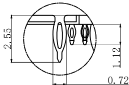
DETAIL B SCALE 5:1 QUANTITY:17
