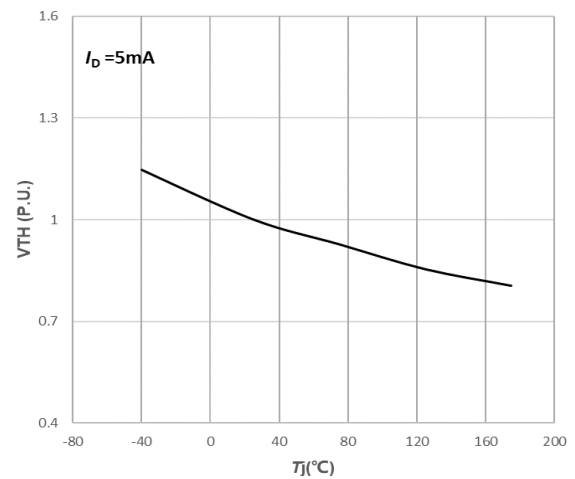
Fig10. Normalized Threshold Voltage vs. Temperature
