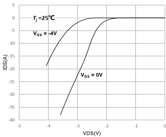
Fig9. Body Diode Characteristics
