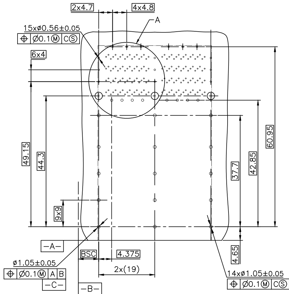
RECOMMENDED PC BOARD LAYOUT COMPONENT SIDE OF BOARD (PCB TOLERANCE:±0.05)
