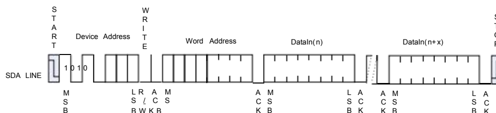
Figure 5-2 Page Write
