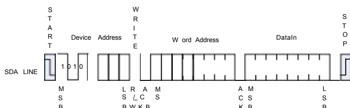
Figure 5-1 Byte Write
