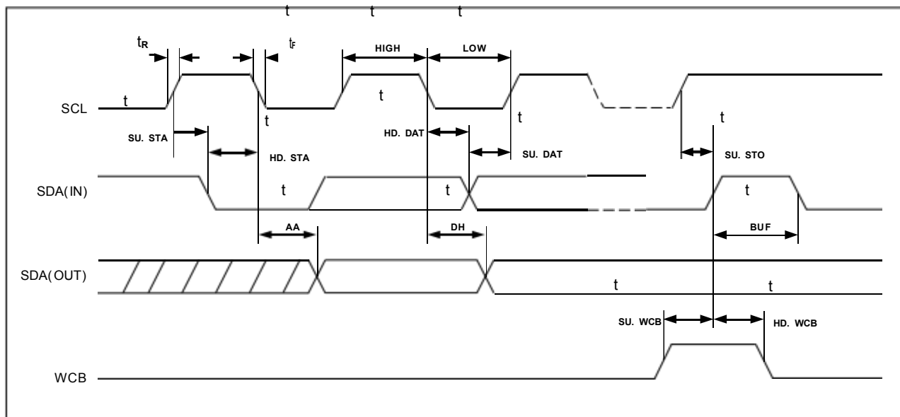
Figure 3-1 Bus Timing
