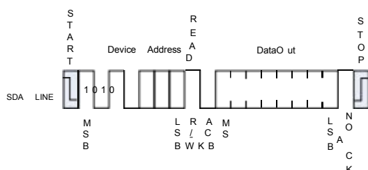
Figure 5-3 Current Address Read
