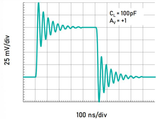
Small Signal Step Response (500 mV).
