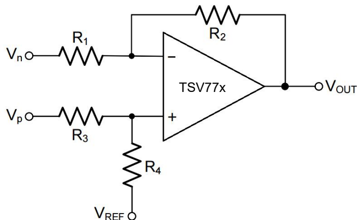
Figure 8. Differential Amplifier
