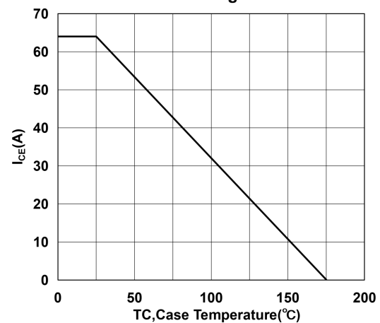
Maximum Collector-Emitter Current Standard Derating Curve
