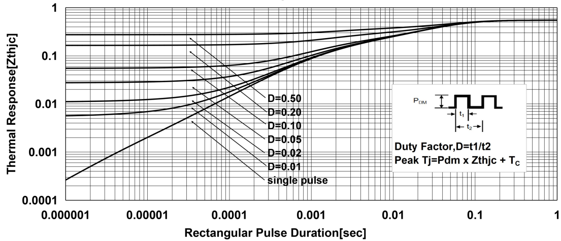
Transient Thermal Impedance of IGBT
