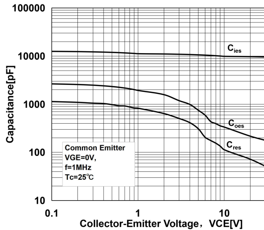
Capacitance Characteristics
