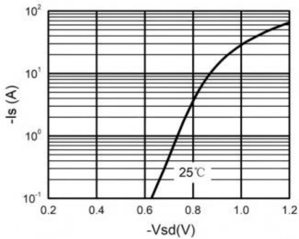
Figure 9. Body-Diode Characteristics
