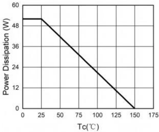
Figure 3. Power Dissipation
