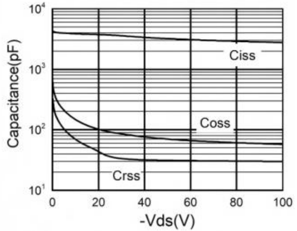
Figure 8. Capacitance
