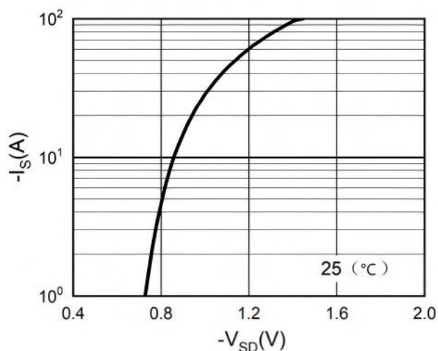
Figure 9. Body-Diode Characteristics
