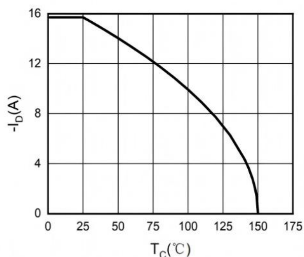
Figure 4. Drain Current
