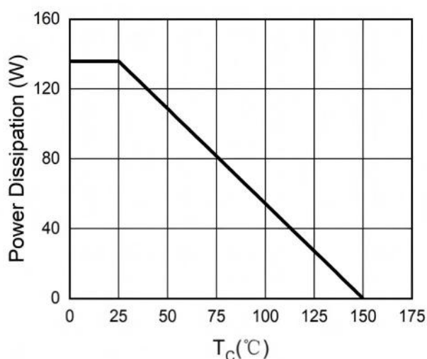
Figure 3. Power Dissipation
