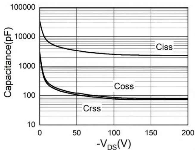
Figure 8. Capacitance
