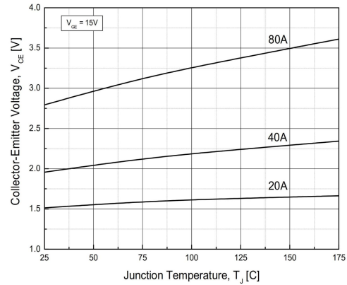
Fig.4 Typical Collector-Emmitter Saturation Voltage -Junction Temperature
