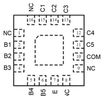
QFN-16 3*3
