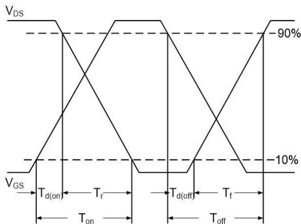
Fig.10 Switching Time Waeform
