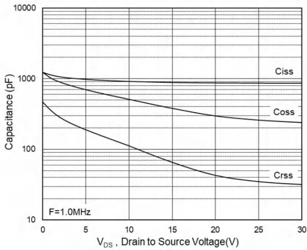
Fig.7 Capacitance
