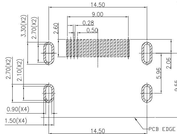
RECOMMENDED PCB LAYOUT(TOP VIEW) (THICKNESS=1.6 \pm 0.05mm)
