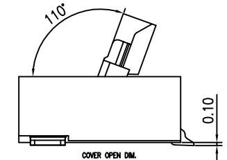
COVER OPEN DIM. SCALE 2:1
