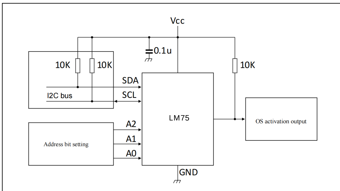
Figure 8. Typical Application
