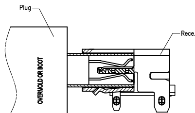
Mated Condition
