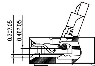
COVER OPEN DIM. SCALE 2:1
