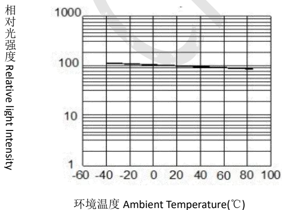
Relative Light Intensity vs. Ambient Temperature
