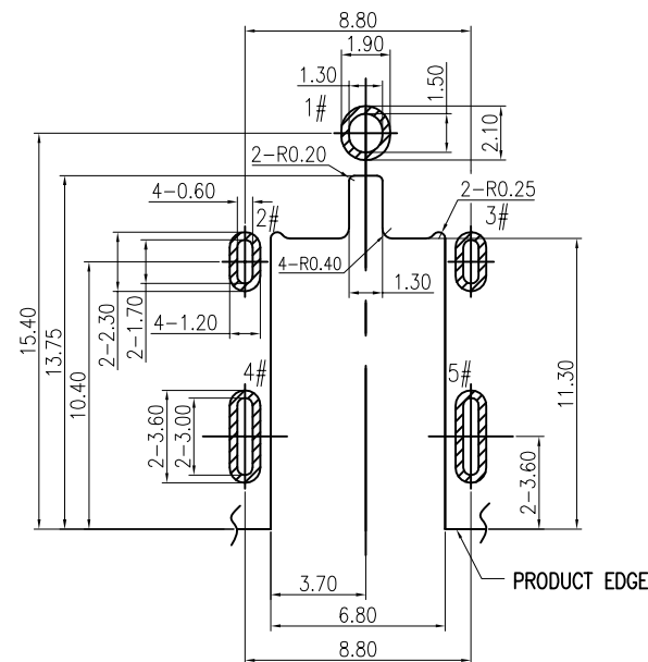
RECOMMENDED PCB LAYOUT(t=1.00) TOP VIEW TOLERANCE:±0.05
