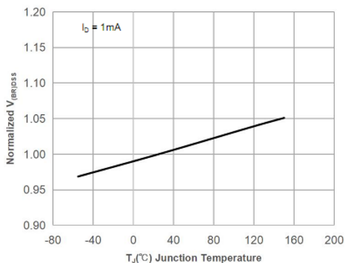
Figure 7: Normalized Breakdown voltage vs. Junction Temperature
