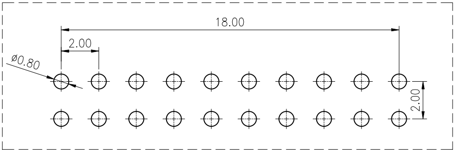
PCB LAYOUT General±0.05mm.
