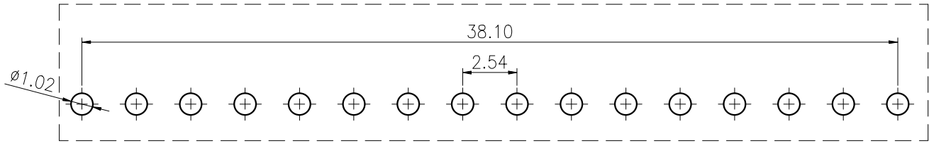
PCB LAYOUT
