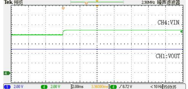
Line Transient (8V to 9V)
