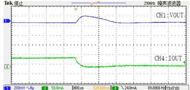
Load Transient (50mA to 150mA)
