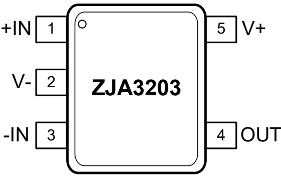
Figure 2. ZJA3203 Pin Configuration (5-lead SOT23)
