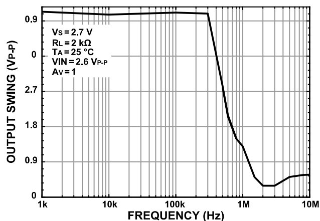
Figure 30. Close-Loop Output Swing vs. Frequency
