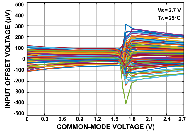
Figure 26. Input Offset vs. Common-Mode Voltage
