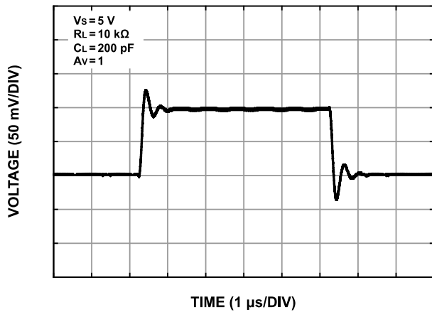
Figure 23. Small Signal Transient Response
