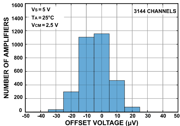
Figure 6. Input Offset Voltage Distribution
