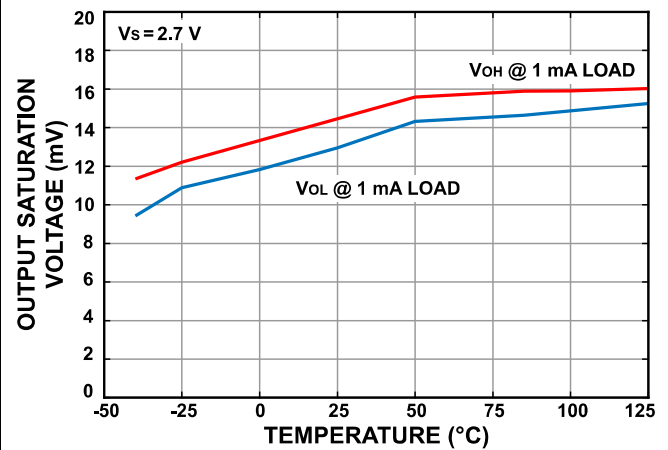
Figure 28. Output Saturation Voltage vs. Temperature
