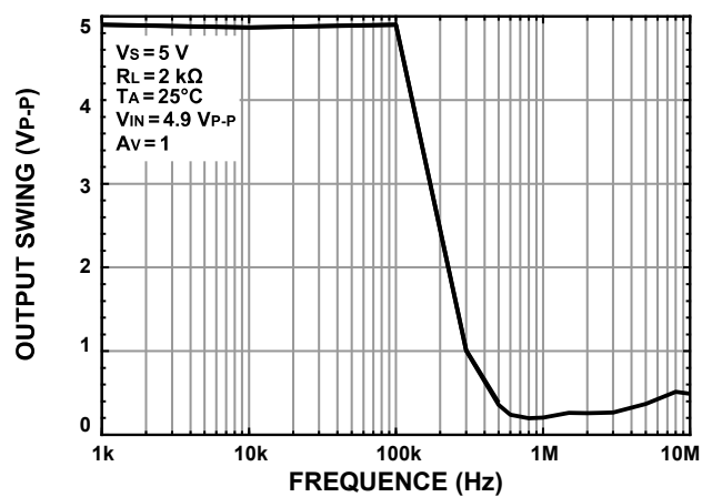
Figure 13. Close-Loop Output Swing vs. Frequency
