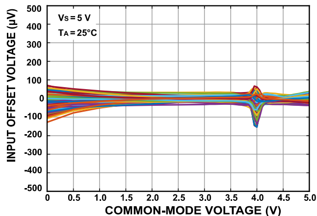
Figure 8. Input Offset vs. Common Mode Voltage
