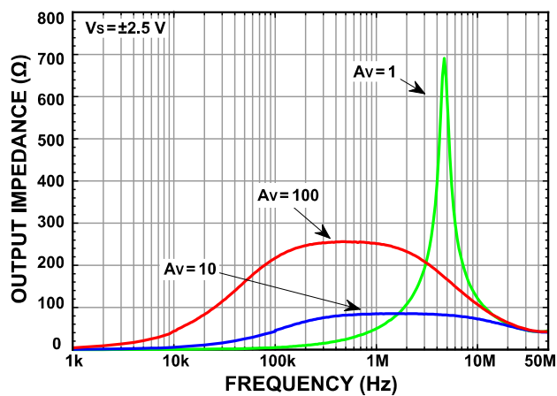
Figure 14. Output Impedance vs. Frequency
