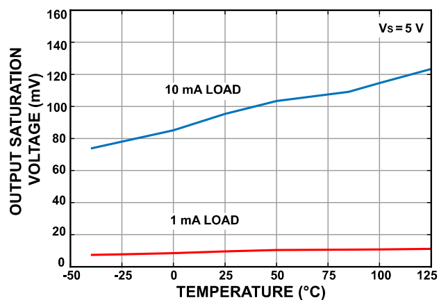
Figure 11. Output Saturation Voltage vs. Temperature
