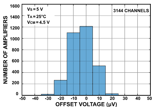
Figure 7. Input Offset Voltage Distribution
