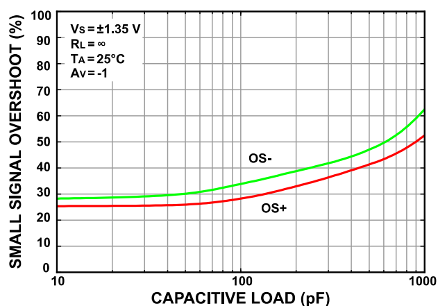
Figure 31. Small-Signal Overshoot vs. Load Capacitance
