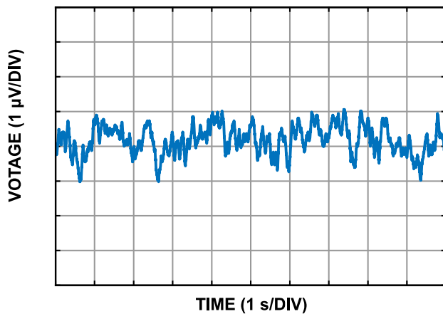
Figure 25. 0.1 Hz to 10 Hz Input Voltage Noise
